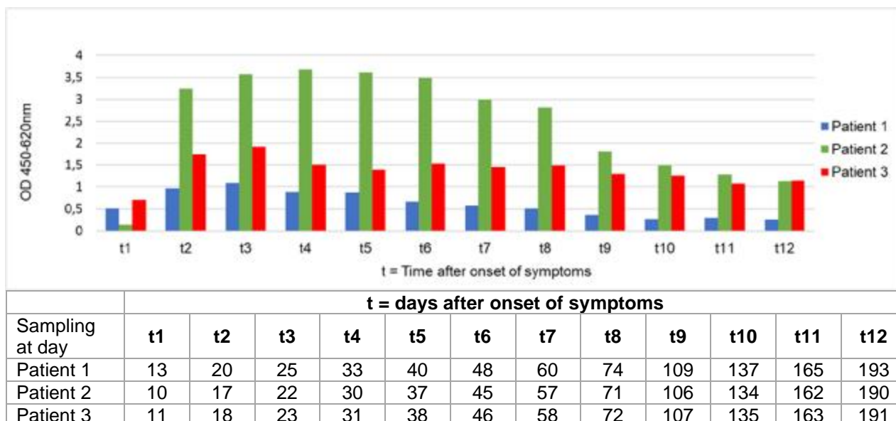
Fig. 2: Time course of IgM-antibody development against SARS-CoV-2-S1 (RBD) protein of three clinically ill patients
